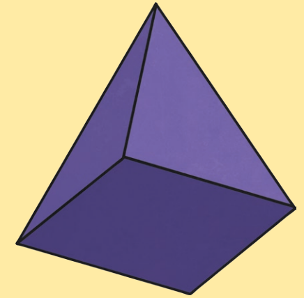
Square-based Pyramid
